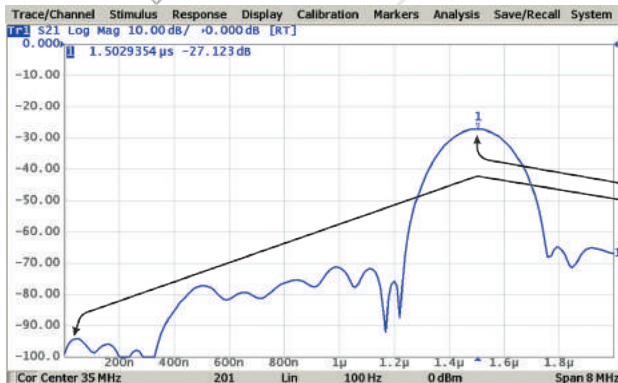
Time domain analysis allows measurements of SAW filters such as the time delay and feedthrough signal suppression.
