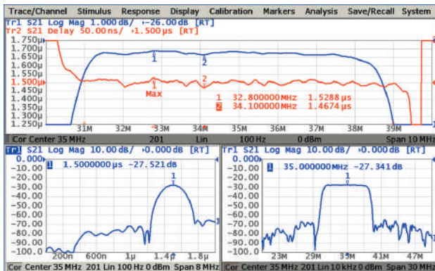
Time domain analysis allows measurements of SAW filters such as the time delay and feedthrough signal suppression.
